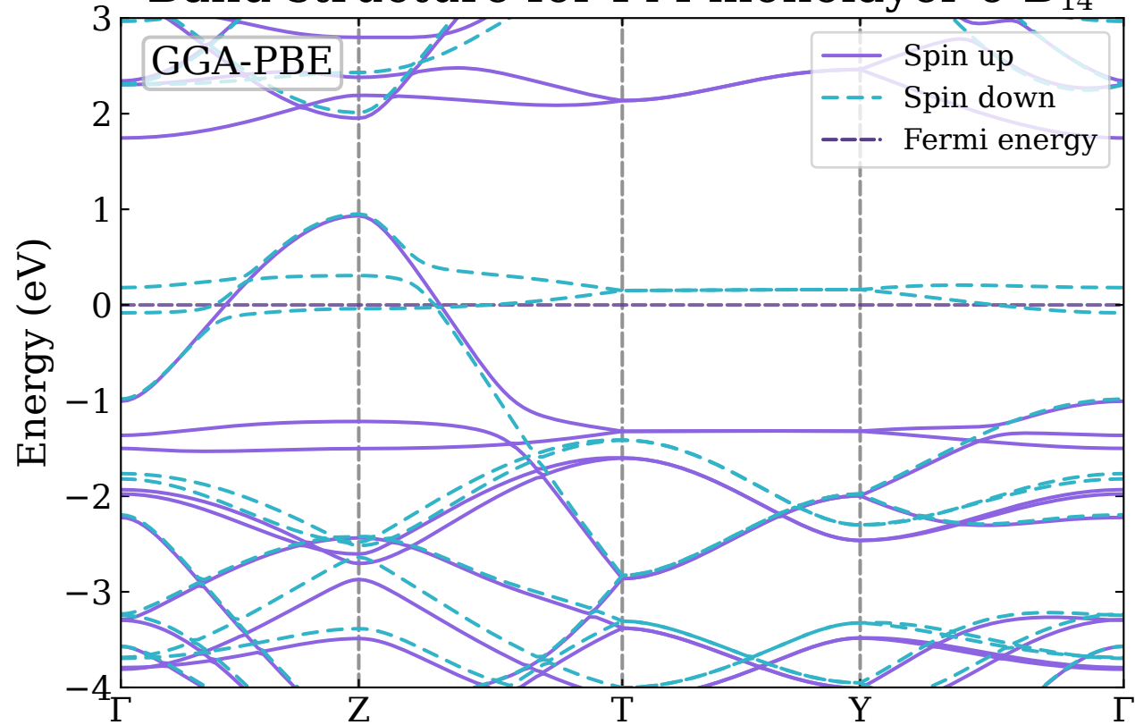
Band structure for FM monolayer o-B 14
