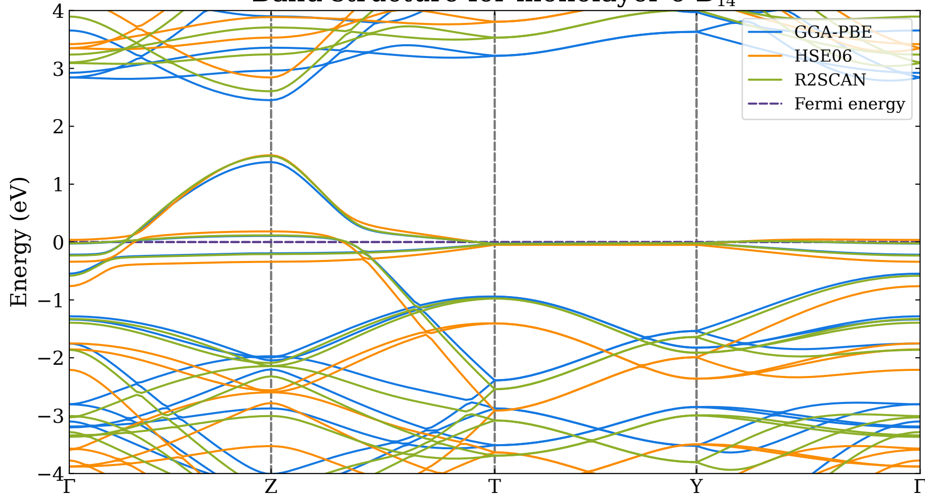
Band structure for monolayer o-B 14
