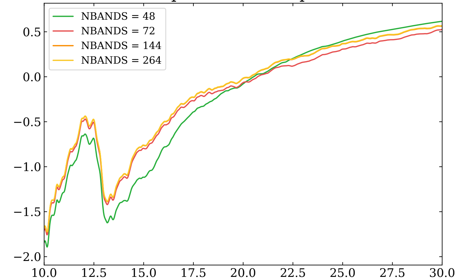
Real part for zz-component
