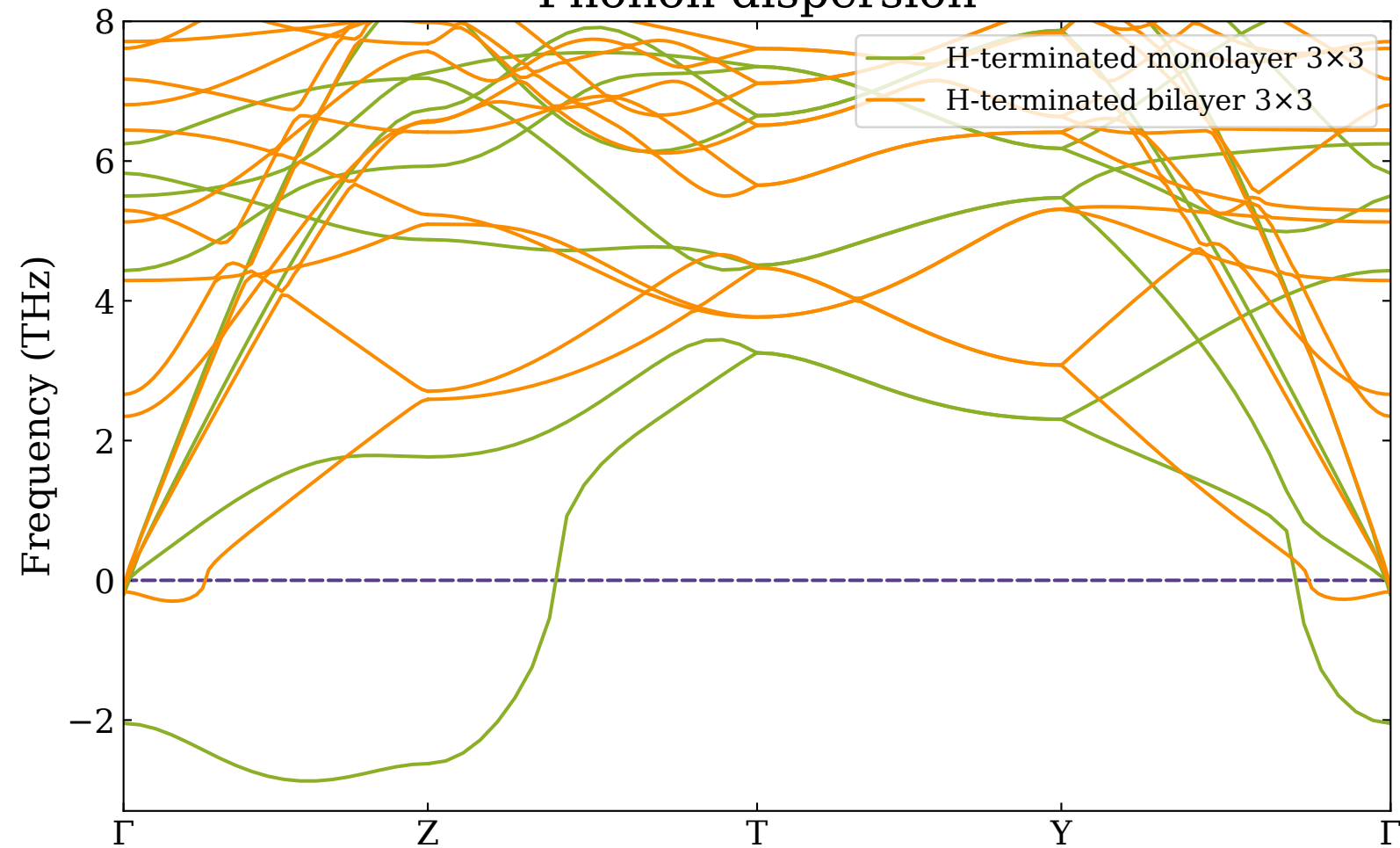
Phonon dispersion
