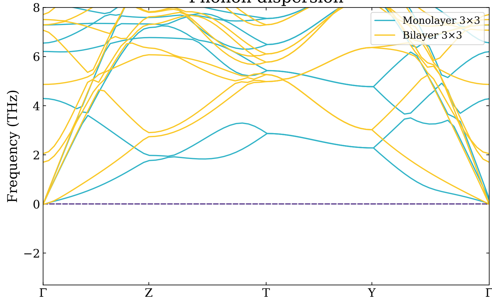
Phonon dispersion
