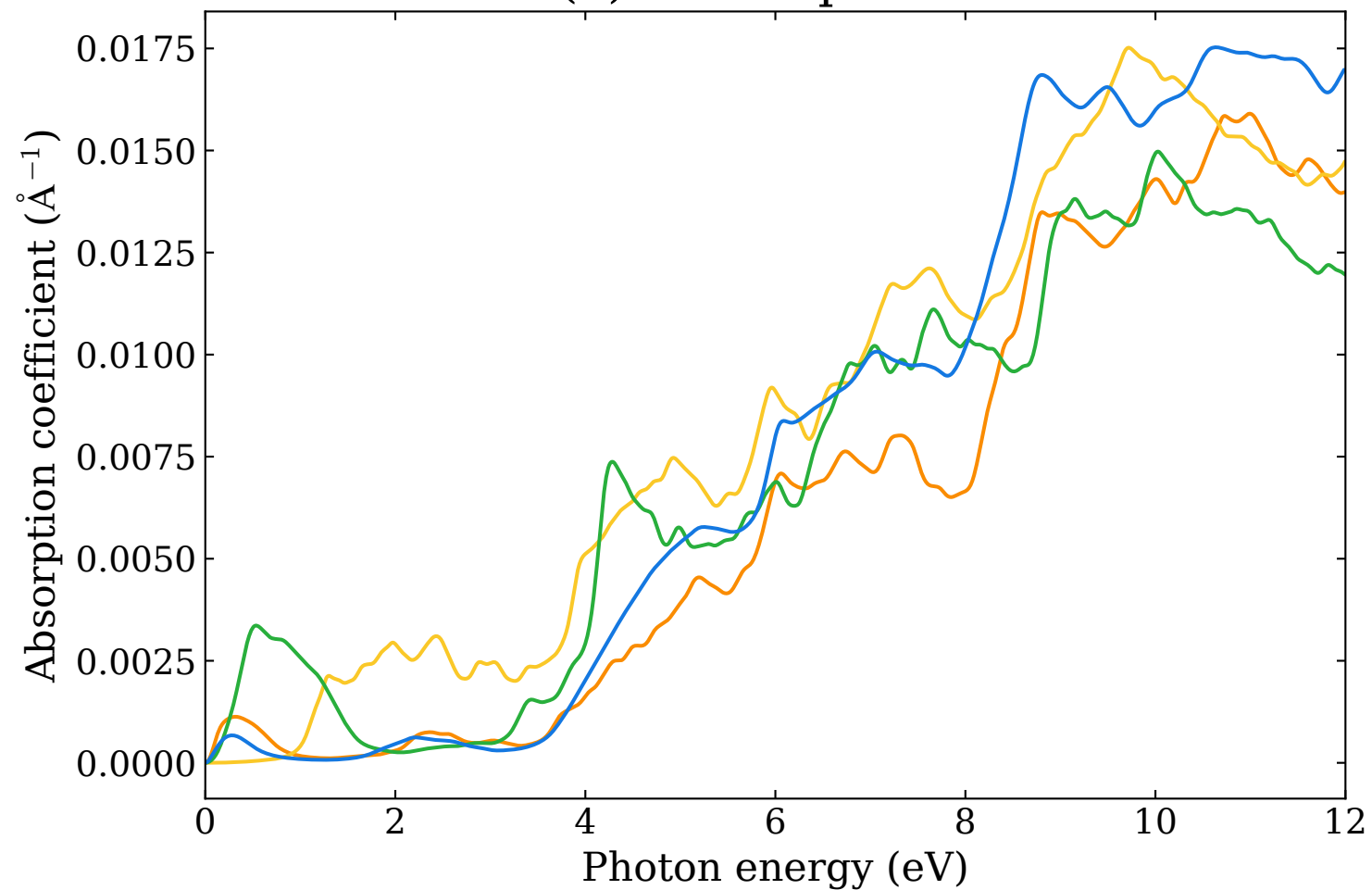
(a) xx-component
