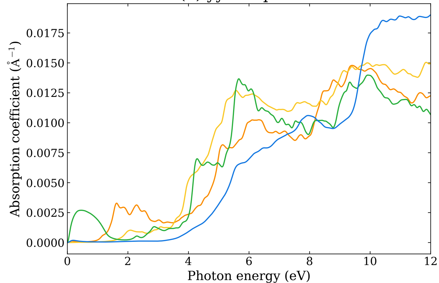
(b) yy-component
