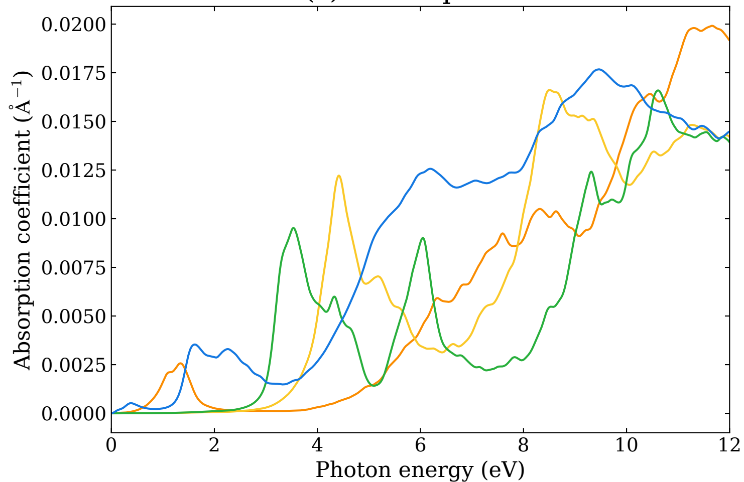
(c) zz-component
