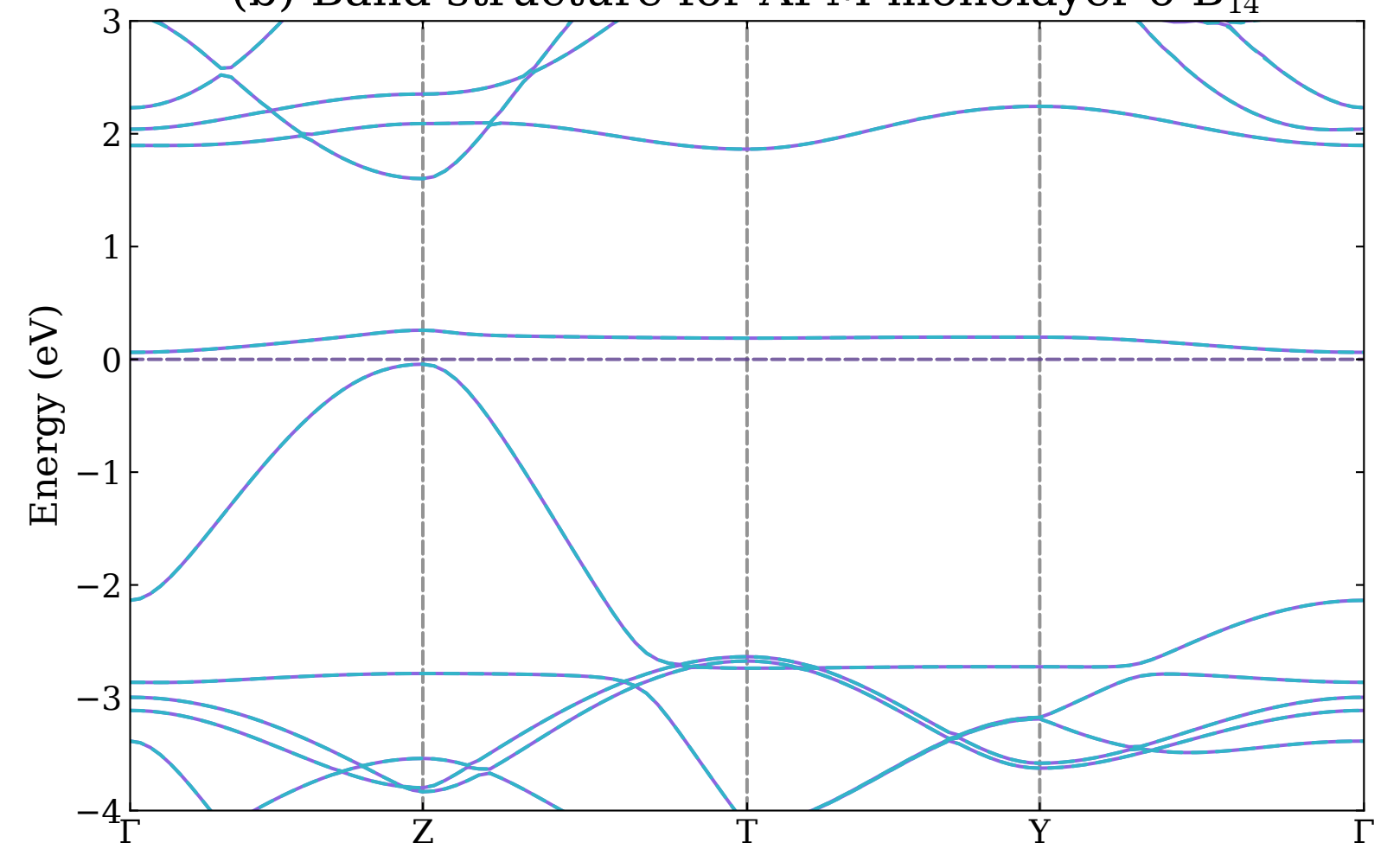
(b) Band structure for AFM monolayer o-B 14
