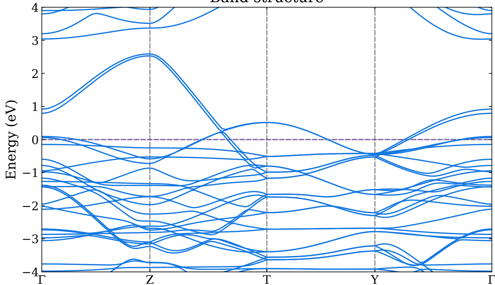
Band structure
