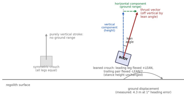
Directional hopping thrust-vector schematic
