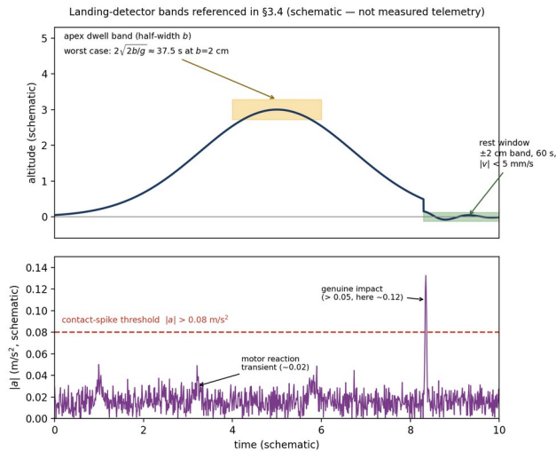
Fig. 10 sketches these bands schematically against a representative hop.
