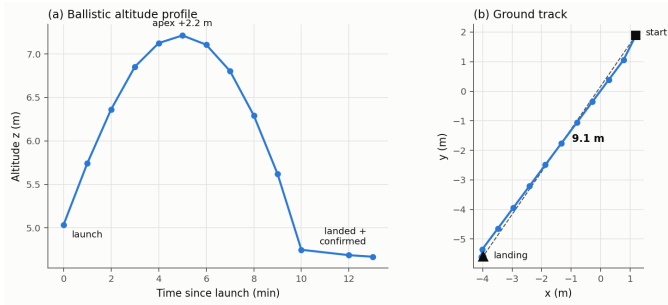
Fig. 13. Measured single-hop trajectory from odometry telemetry — (a) the ballistic altitude profile over a multi-minute flight and (b) the straight-line ground track.
