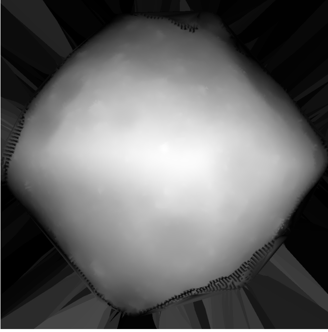
Fig. 1. Lateral X-axis projection heightmap derived from the Hayabusa2 SfM shape model, detailing Ryugu’s equatorial ridge.
