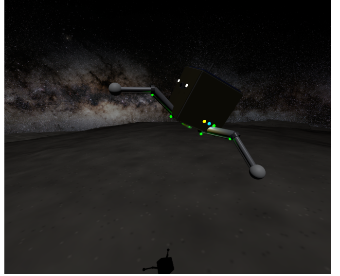
Fig. 5. A scout mid-hop. The forward lean is visible in the body attitude; the shadow on the regolith below shows the altitude gained within seconds of the stroke.
