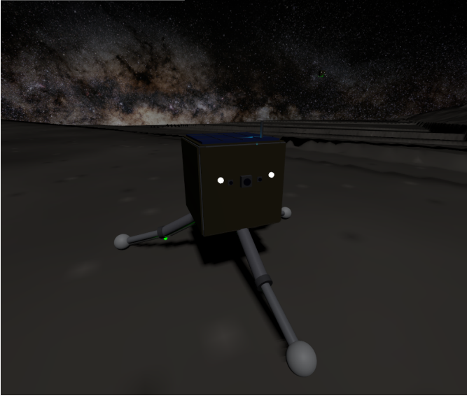
Fig. 4. The SpaceHopper model — face-on view showing the stereo hazard cameras and navigation camera, UHF antenna, solar array, and the tri-pedal articulated legs with spherical feet.
