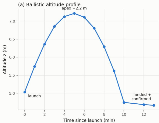
Fig. 17. Measured single-hop trajectory from odometry telemetry — (a) the ballistic altitude profile over a multi-minute flight and (b) the straight-line ground track. * Flight stabilization: in-flight body rates damped to 0.005–0.015 rad/s; launch transients of 0.24 rad/s removed within seconds; no persistent yaw spin. A commanded 107^\circ yaw slew converged overdamped and held within 1^\circ at zero rate; a 165^\circ tumble was damped to 3.6^\circ in \sim 20 s. * Self-righting (tilt-dependent, honestly characterized). A dedicated re-verification exposed, and then drove the redesign of, the reaction-wheel righting maneuver (§3.3). The pre-redesign maneuver succeeded in only 5 of 21 attempts (24%) over a long run: inverted bodies rolled onto their side and stalled there, and each failure triggered a spurious low-velocity liftoff that sent the robot on an uncommanded multi-minute-to-hour re-flight — the parasitic cascades that dominated earlier runs. The redesigned maneuver (direction-aware roll, proportional-taper speed, tuck-then-deploy legs) eliminates that stall. Its reliability was then measured directly by teleporting resting robots to controlled inversions and scoring recovery, and the result is genuinely tilt-dependent, so it is reported as such rather than as a single figure: the mild-to-moderate tilts characteristic of an actual milli-gravity landing recovered reliably (every such case in the sample), while a body forced to a perfect full inversion — balanced on its dome and often wedged against a terrain feature — recovered in only about one case in four , the residual failure being a physically-trapped configuration that internal reaction-wheel actuation cannot roll out of. A successful roll completes in a few seconds of active rolling; multi-attempt sequences take longer. This is a substantial, measured improvement over the 24% baseline, honestly bounded: the platform reliably rights the tilts it actually incurs, and does not claim to recover every adversarial inversion. * Landing: decaying-bounce settle and confirmed LANDED in \sim 14 min after a full-stroke hop; no false confirmations in flight and no post-landing self-ejection across the final verification runs. * Swarm autonomy (3 agents): differentiated role allocation on first boot (RELAY + 2\times SCOUT), competitive auctions on detected anomalies, dispatch, range-matched directional hops, and cooldown-paced corrective re-hops — the full loop operating without operator intervention. * Sampling cycle: on a SAMPLER reaching its anomaly (arrival check against live odometry, 0.9 m from target on the verified run), the swarm layer autonomously deployed the core drill, completed the extraction dwell, stowed the core in carousel tube 1/3, and immediately re-tasked the agent to its next queued anomaly
