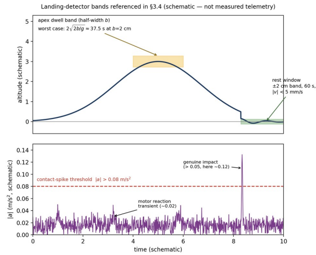
Fig. 10. Landing-detector bands referenced above — the contact-spike acceleration threshold and the apex-dwell/rest-window altitude bands (schematic, not measured telemetry).
