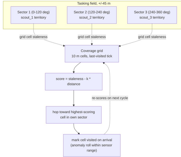
Fig. 16. Search algorithm data flow. Each agent scores candidate cells only within its own static sector, so the three searches never compete for the same ground.
