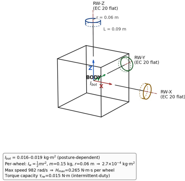
Fig. 7. Reaction-wheel layout and moment-of-inertia axes, isometric engineering sketch with dash-dot centerlines and a dimensioned wheel (not to scale; not a CAD render).
