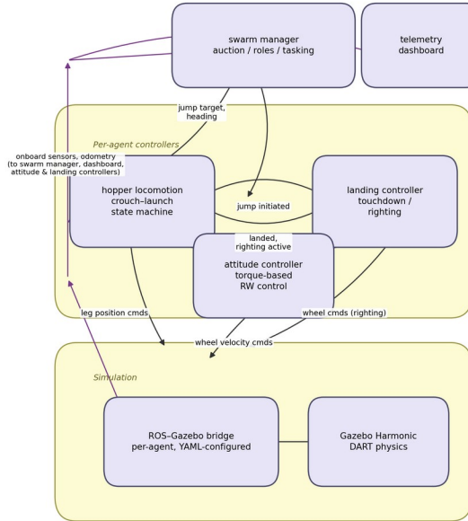
Fig. 3. System architecture. The landed and righting_active flags implement strict actuator arbitration — exactly one node commands any actuator at any time (§8).
