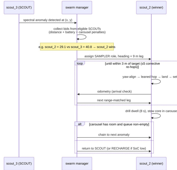
Fig. 15. Auction-based tasking and sampling sequence, as executed live by the three-agent swarm.
