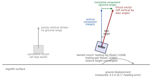
Fig. 5. Directional hopping schematic — the leaned crouch tilts the launch thrust vector off vertical, splitting delta-v into a vertical (height) and horizontal (ground-range) component, aimed by reaction-wheel yaw-hold.
