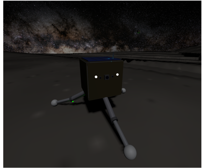
Fig. 4. The SpaceHopper model — face-on view showing the stereo hazard cameras and navigation camera, UHF antenna, solar array, and the tri-pedal articulated legs with spherical feet.
