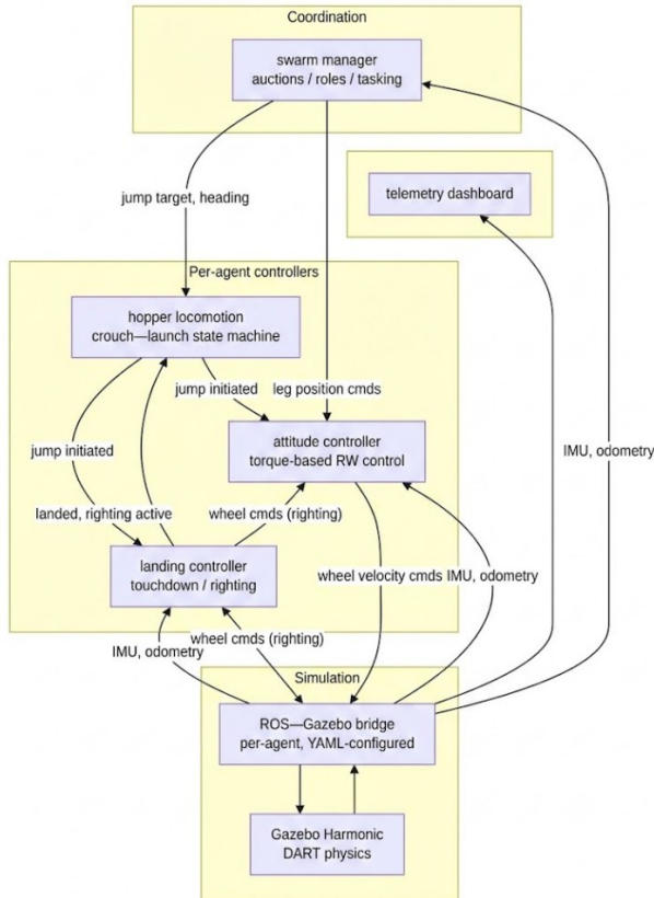
Figure 3: System architecture. The landed and righting_active flags implement strict actuator arbitration: exactly one node commands any actuator at any time (§8).
