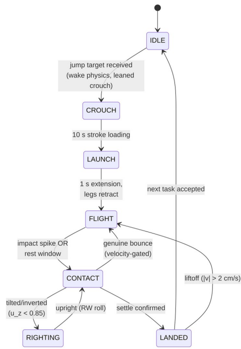
Figure 12: The hop–land–right cycle. Attitude control runs during FLIGHT (motion-gated), stands down during RIGHTING , and holds yaw only when grounded.
