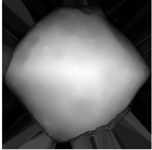
Figure 1: Lateral X-axis projection heightmap derived from the Hayabusa2 SfM shape model, detailing Ryugu’s equatorial ridge.
