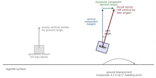
Figure 5: Directional hopping schematic: the leaned crouch tilts the launch thrust vector off vertical, splitting delta-v into a vertical (height) and horizontal (ground-range) component, aimed by reaction-wheel yaw-hold.
