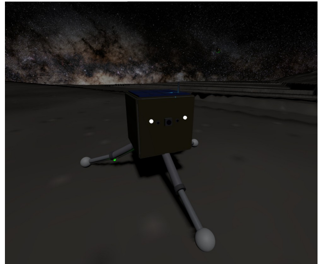
Figure 4: The SpaceHopper model, face-on view showing the stereo hazard cameras and navigation camera, UHF antenna, solar array, and the tri-pedal articulated legs with spherical feet.
