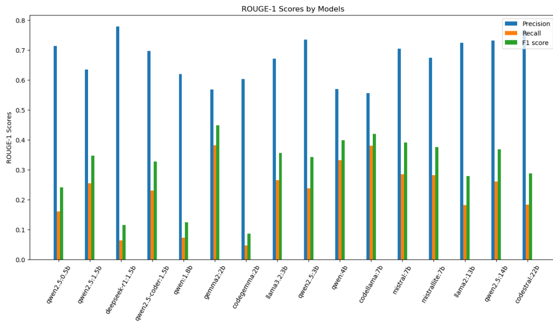
Figure B.1: ROUGE-1 Scores by LLMs.
