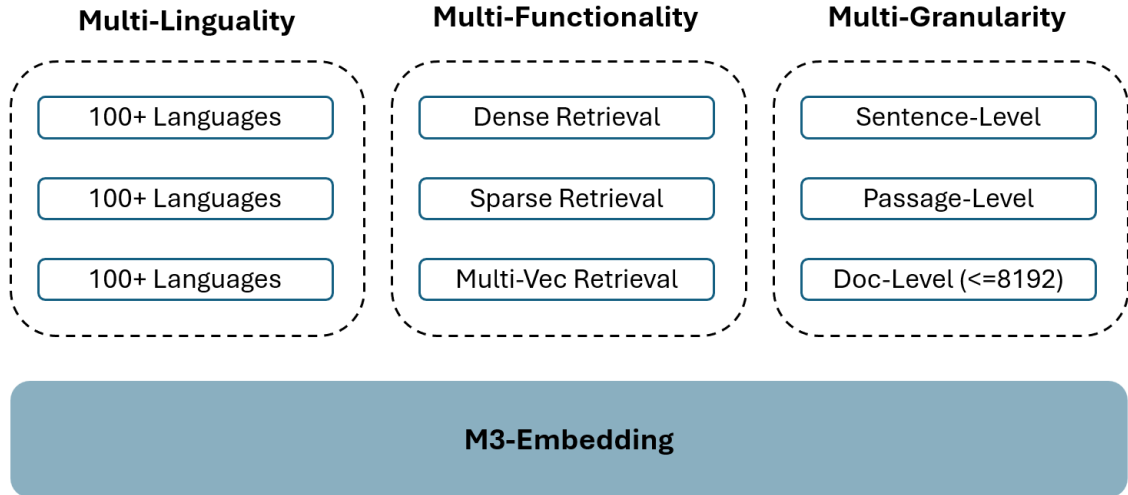
Figure 3.5: Characters of M3-Embedding [chen2024bge].
