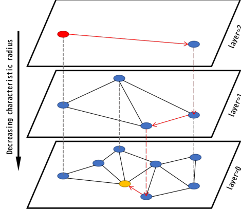
Figure 2.3: HNSW search algorithm visualization. The search starts from entry point from top layer (shown red), red arrows show direction of greedy algorithm to query point (shown yellow) [malkov2018hnsw].
