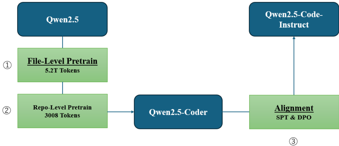
Figure 3.8: The three-stage training pipeline for Qwen2.5-Coder [hostnik2024].
