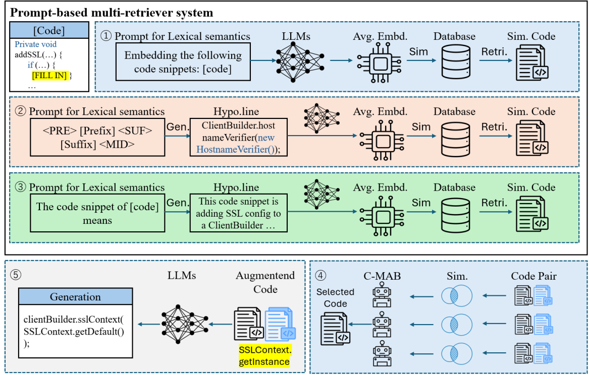
Figure 3.4: ProCC framework [tan2024].
