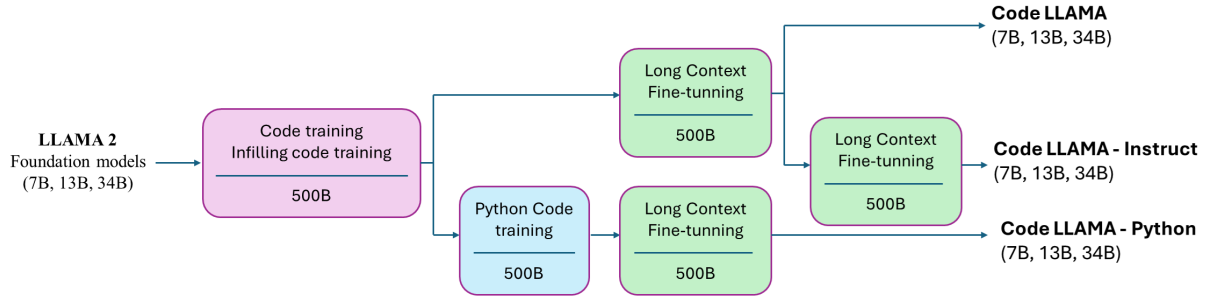
Figure 3.6: The Code Llama specialization pipeline [roziere2023code].
