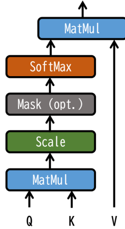
Figure 2.5: Scaled Dot-Product Attention [vaswani2017].
