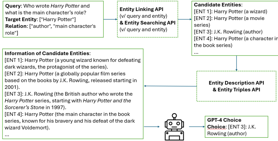
Figure 2.8: Workflow of augmentation with structured data sources [wang2023knowledgpt].
