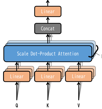
Figure 2.6: Multi-Head Attention (consists of several attention layers running in parallel) [vaswani2017].
