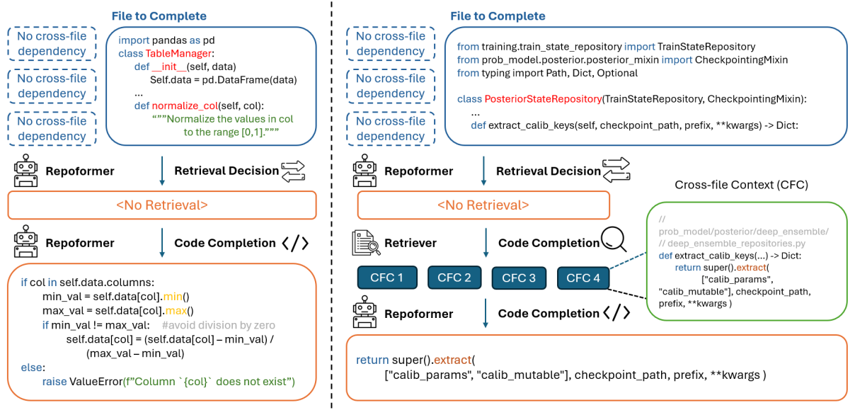
Figure 3.3: REPOFORMER framework [wu2024].
