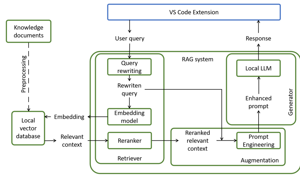
Figure 4.3: Our RAG architecture design
