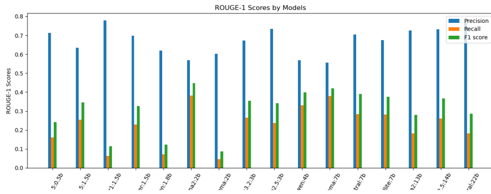
Figure B.1: ROUGE-1 Scores by LLMs.
