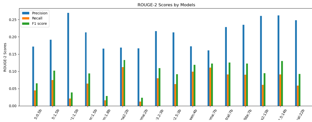
Figure B.2: ROUGE-2 Scores by LLMs.
