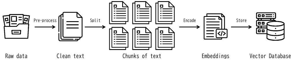
Figure 2.2: Preprocessing process for retriever
