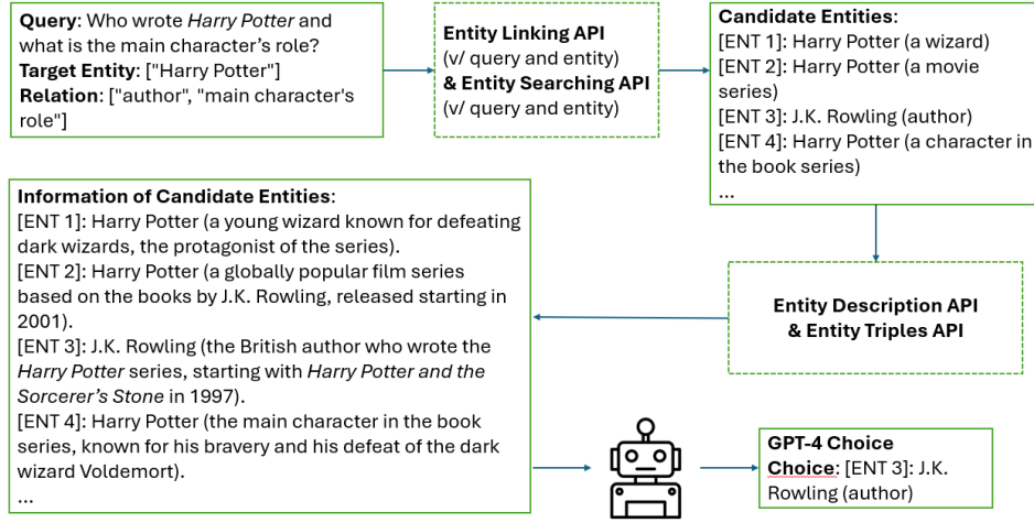
Figure 2.8: Workflow of augmentation with structured data sources [57]
