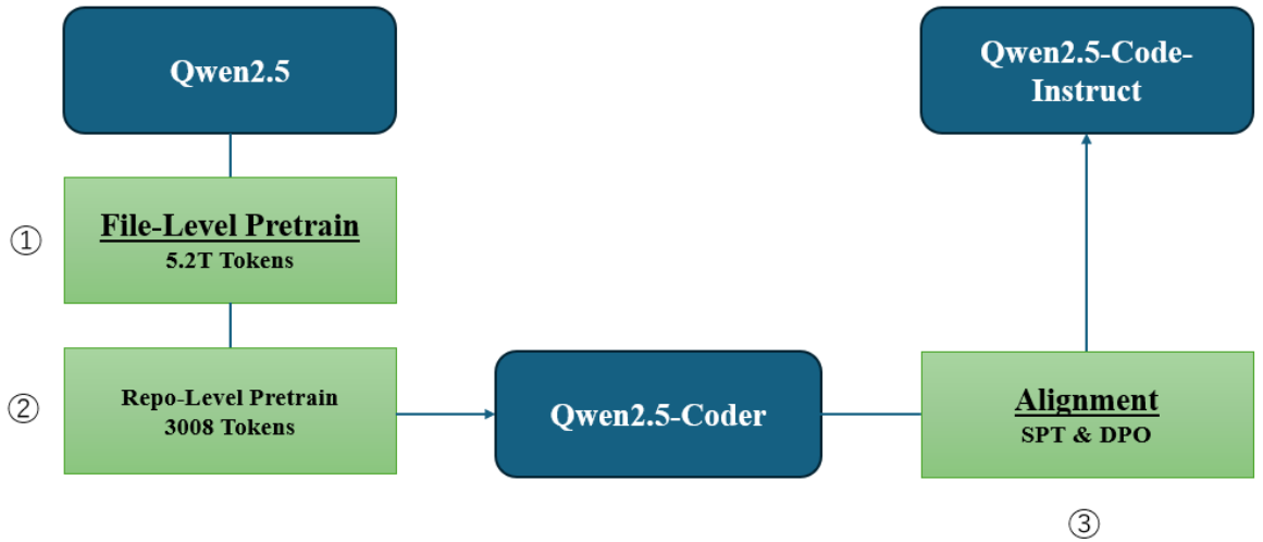
Figure 3.8: The three-stage training pipeline for Qwen2.5-Coder [21]
