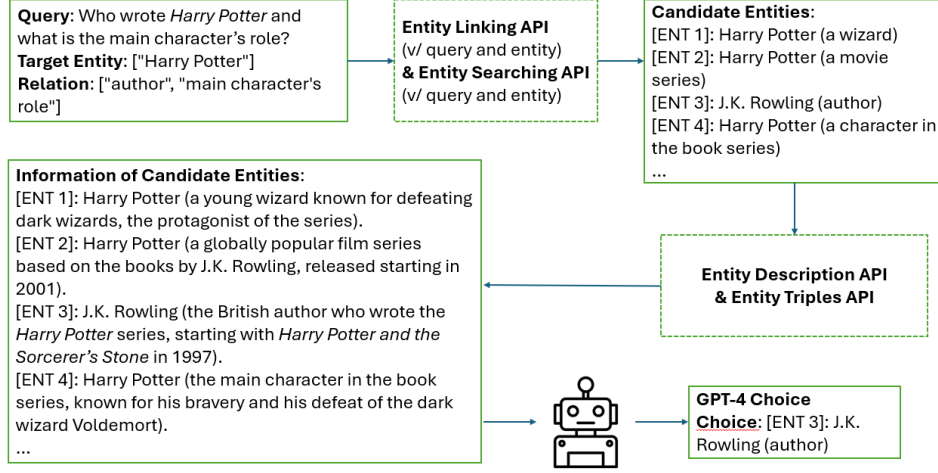
Figure 2.8: Workflow of augmentation with structured data sources [56]
