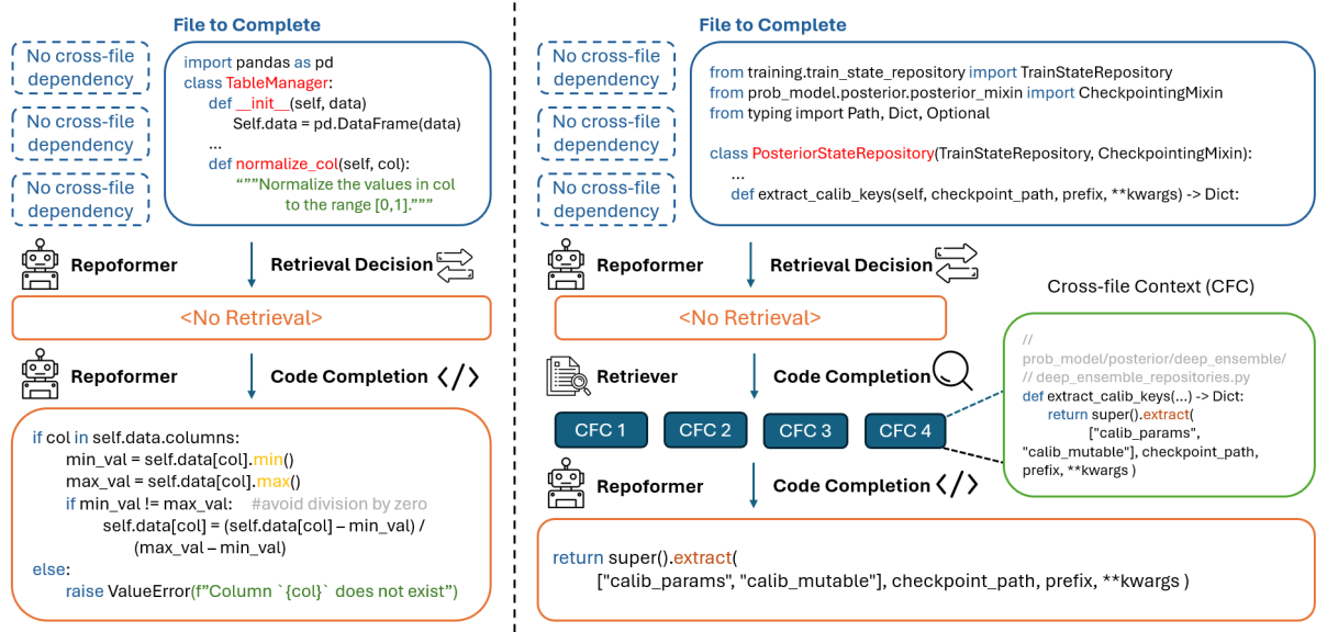
Figure 3.3: REPOFORMER framework [56].
