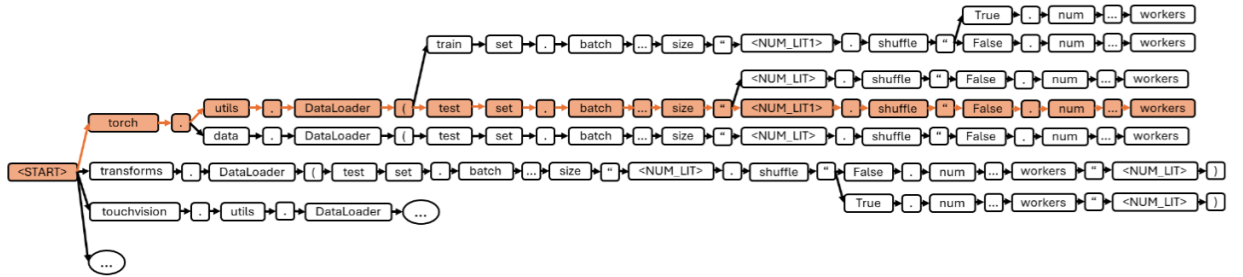
Figure 3.12: IntelliCode Compose’s code snippet completion suggestion and completion-tree demonstration [48]
