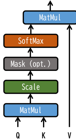
Figure 2.5: Scaled dot-product attention [54]
