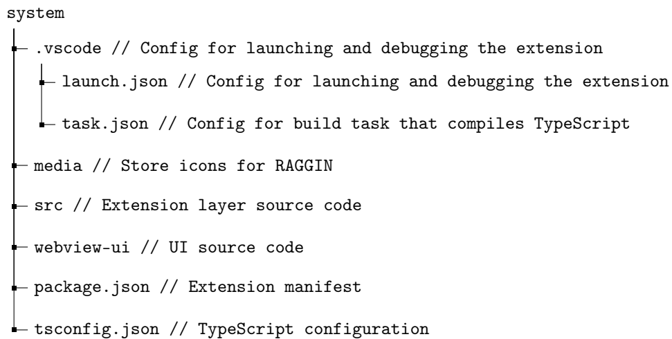
Figure 5.8: RAGGIN codebase directory tree
