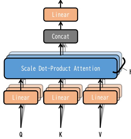
Figure 2.6: Multi-Head Attention (consists of several attention layers running in parallel) [54]
