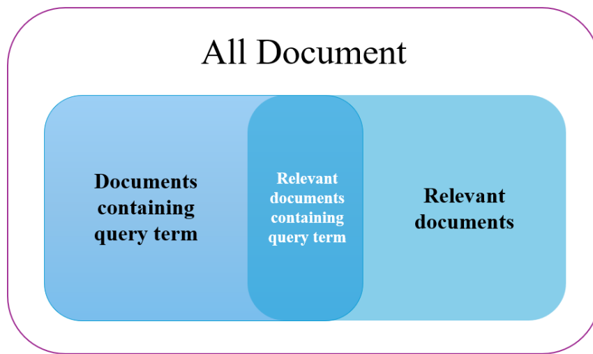
Figure 3.1: BM25 visualization.
