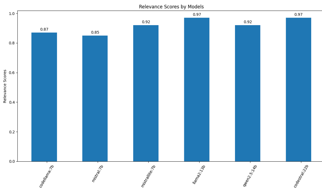
Figure B.6: Relevance Scores by larger LLMs.
