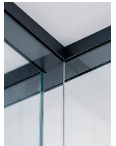
■ Top T-shaped connection 顶部T字连接
