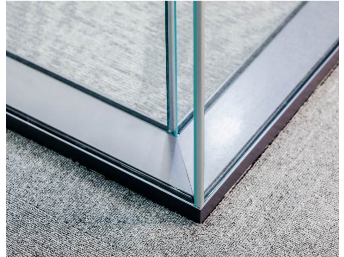
■ L-shaped connection L字连接
