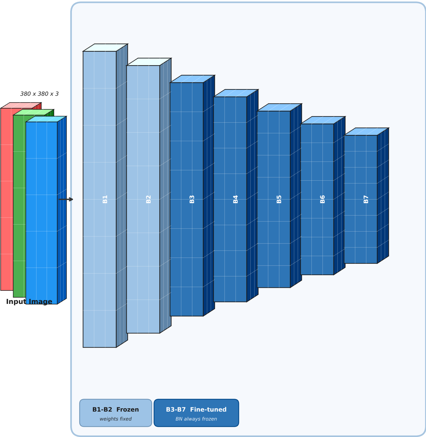
EfficientNetB4 Backbone (ImageNet pretrained)
