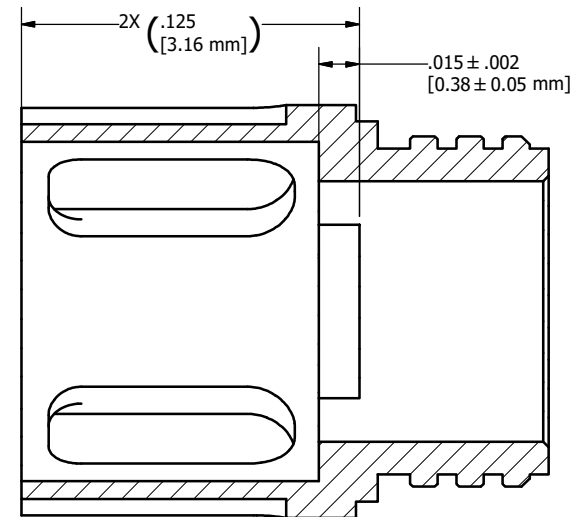
SECTION H-H
