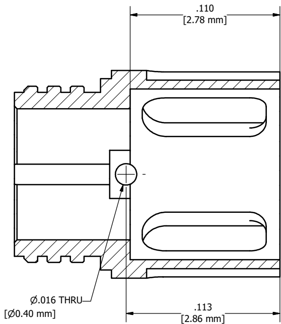
SECTION G-G
