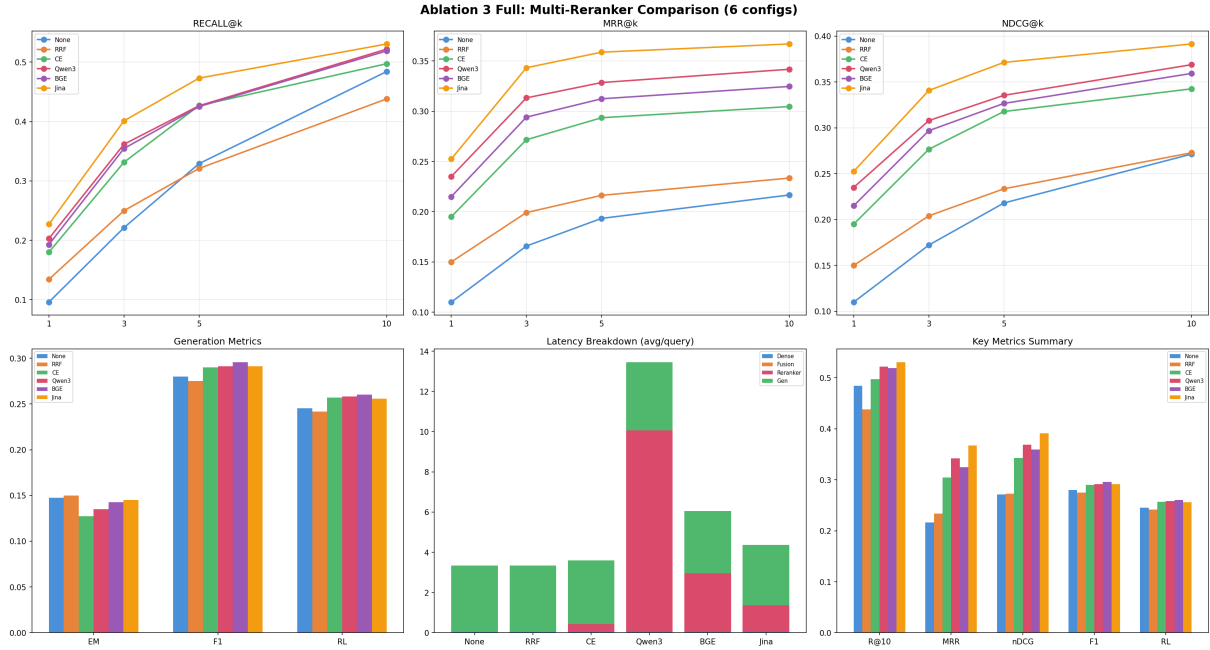
Figure 2: Reranker curves, answer-overlap diagnostics, latency breakdown, and headline metrics from the six-config run. These plots are descriptive; the paired confidence intervals in Table 6 are the primary uncertainty analysis.
