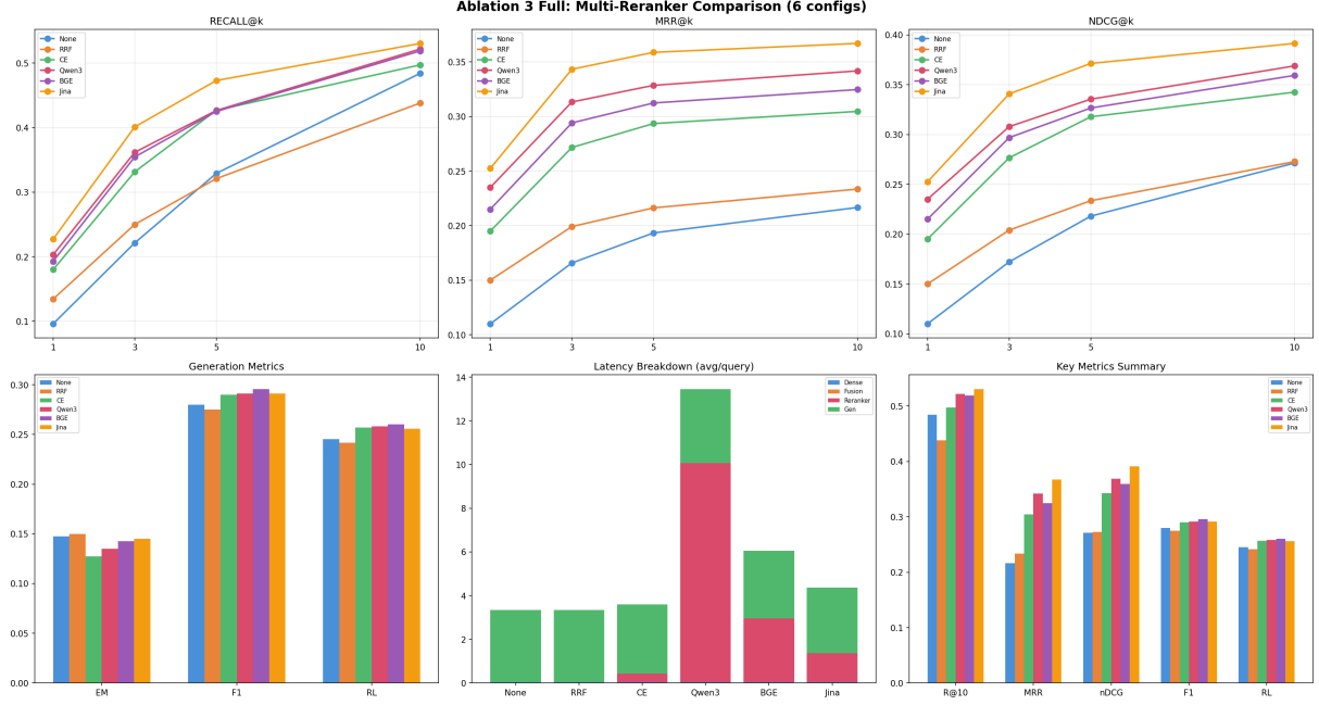
Figure 2: Reranker curves, answer-overlap diagnostics, latency breakdown, and headline metrics from the six-config run. These plots are descriptive; the paired confidence intervals in Table 6 are the primary uncertainty analysis.
