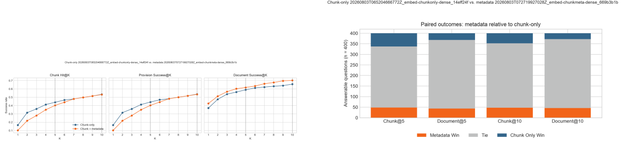
Figure 2: Embedding-text ablation diagnostics. The left panel shows success curves by retrieval depth; the right panel shows paired win, tie, and loss counts. Both plots use the shared answerable-question comparison.
