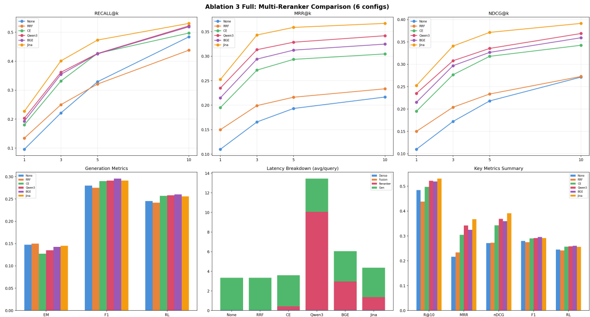
Figure 3: Reranker curves, answer-overlap diagnostics, latency breakdown, and headline metrics from the six-configuration run. The paired confidence intervals in Table 13 are the primary uncertainty analysis.
