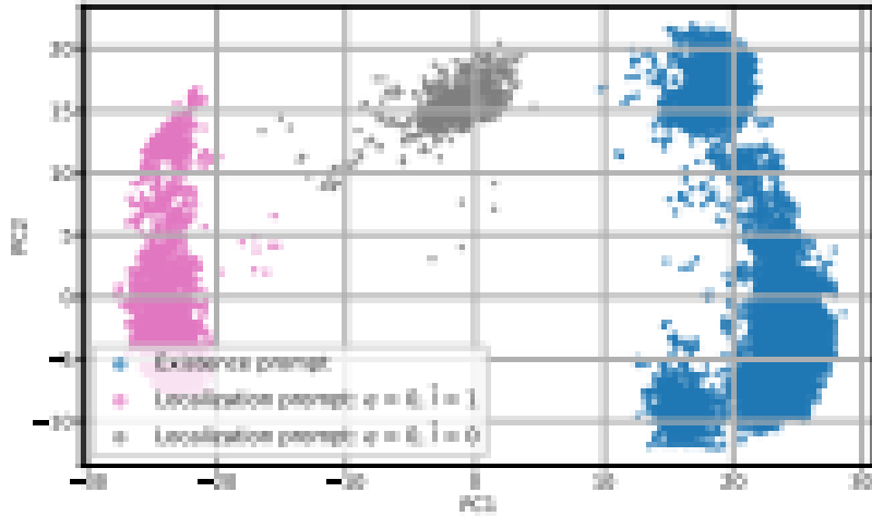
Figure 2: PCA projection of hidden states.
