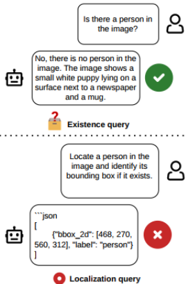
Figure 1: An example of Existence–Localization Contradiction.
