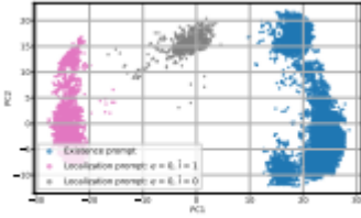
Figure 2: PCA projection of hidden states.
