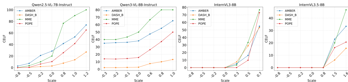
Figure 3: Model performance with different steering coefficients.
