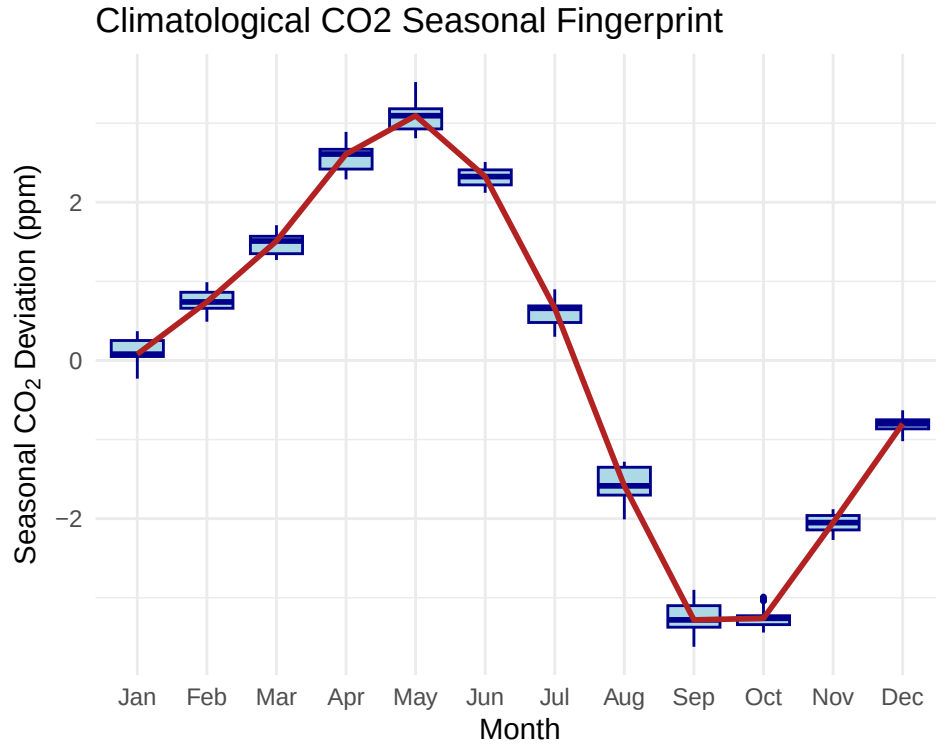
Figure 5: Box plot of seasonal deviations in CO 2 concentrations.
