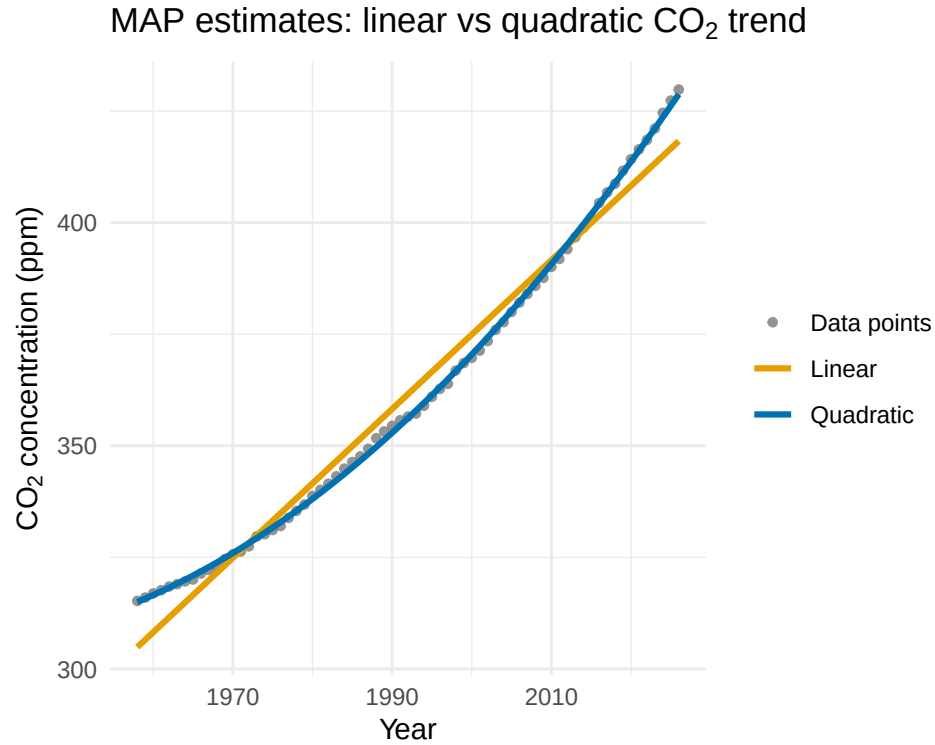
Figure 10: MAP model fits versus observed data. The linear model (orange) and quadratic model (blue) are compared against the yearly average CO2 concentrations. The quadratic fit clearly follows the data more efficiently.
