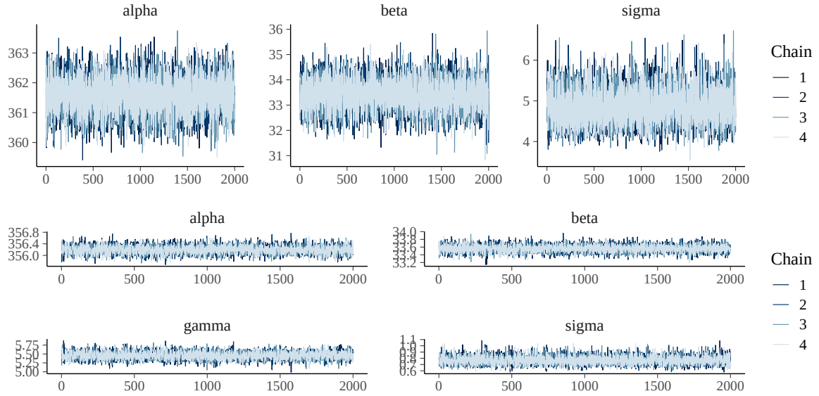
Figure 12: Trace plots for all parameters in all 4 STAN chains. The chains are completely overlapped, demonstrating convergence with \hat{R} = 1 .
