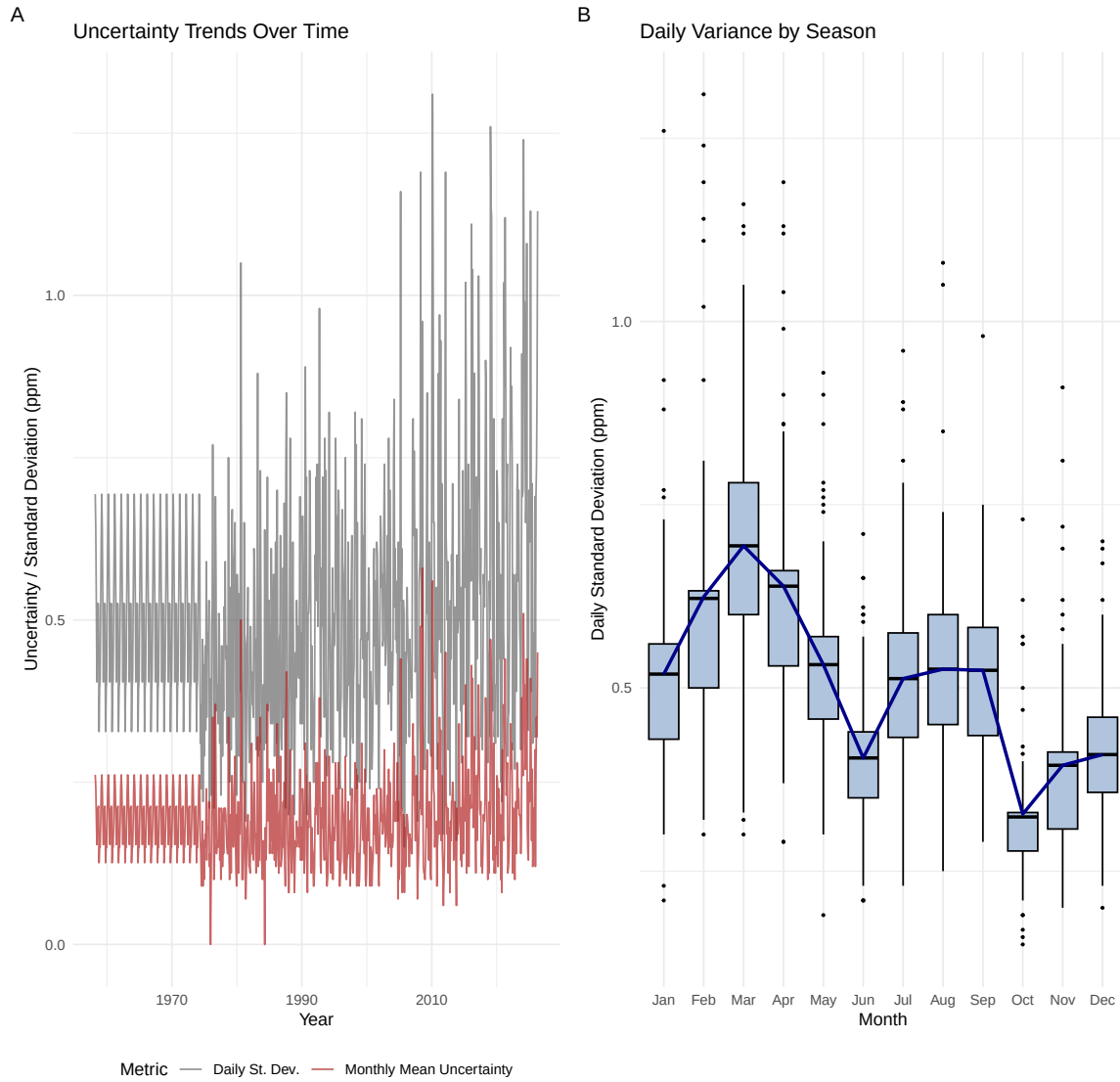
Figure 6: Uncertainty analysis of the CO2 measurements. The left panel shows the trends of daily standard deviation and monthly mean uncertainty over time, while the right panel shows the distribution of daily standard deviation across different months. The oscillation visible in the left panel is due to the use of imputed data for those variables, since their values remain constant across that period of years.
