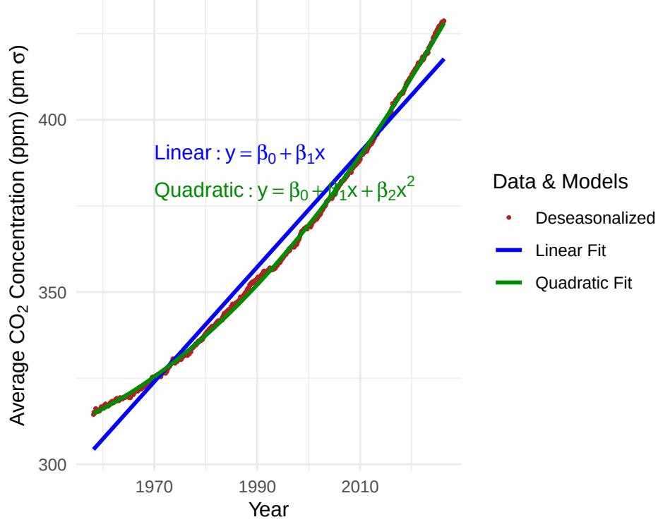
Figure 8: Deseasonalized CO2 concentrations and Bayesian models fit. The plot shows the deseasonalized CO2 concentrations along with the fitted lines from both the linear and quadratic models, illustrating the differences in their respective fits to the data.
