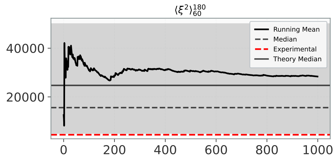
Convergence - base_omegak_CamSpecHM_TT_lowl_lowE
