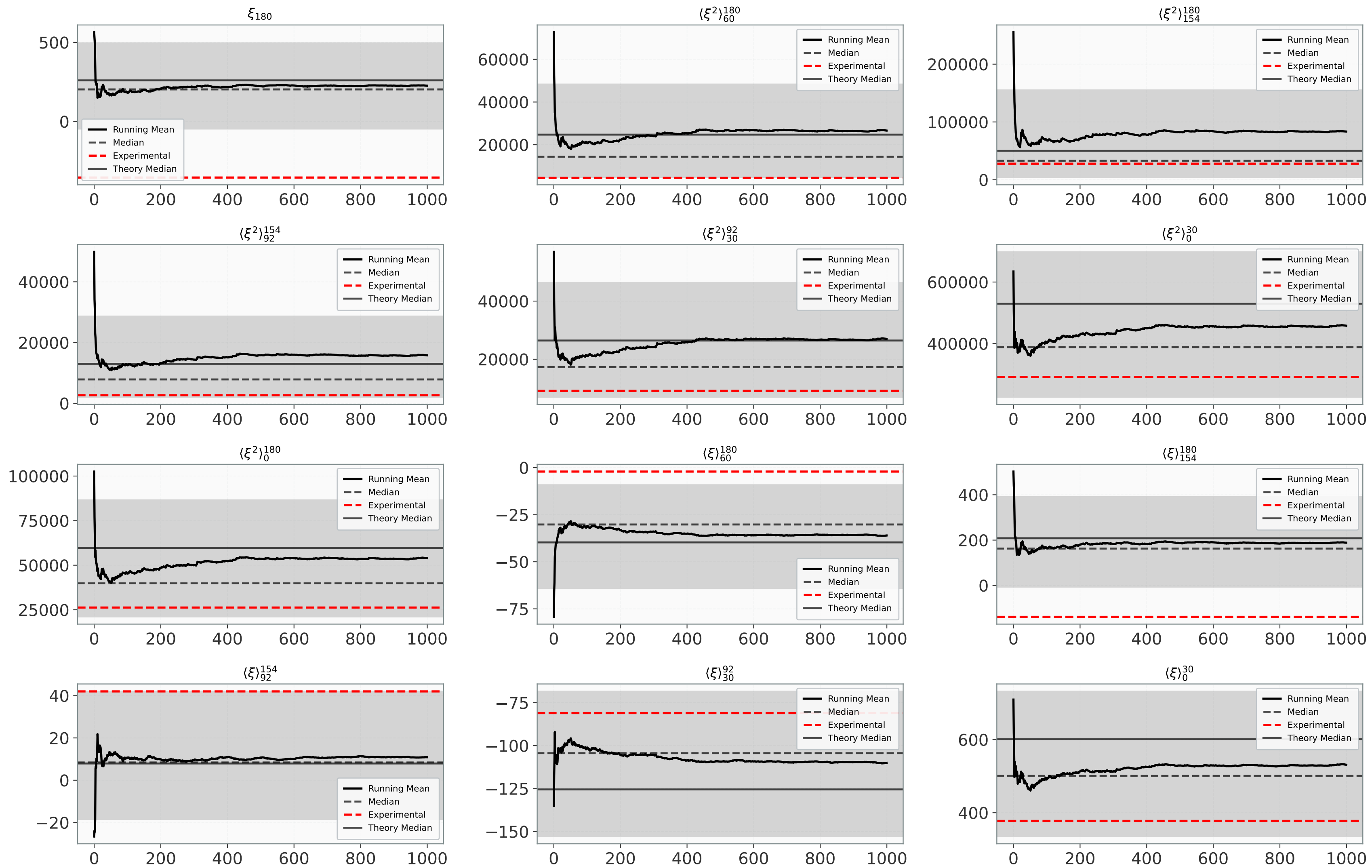
Convergence - base_omgak_plikHM_TTTEEE_lowl_lowE
