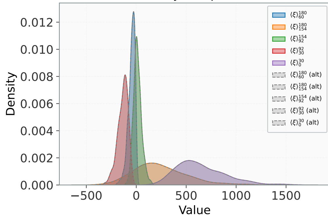
Density Comparison
