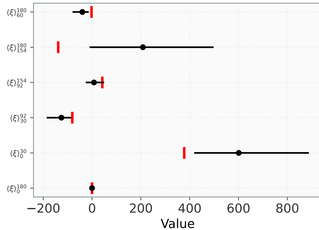
68% Credible Intervals
