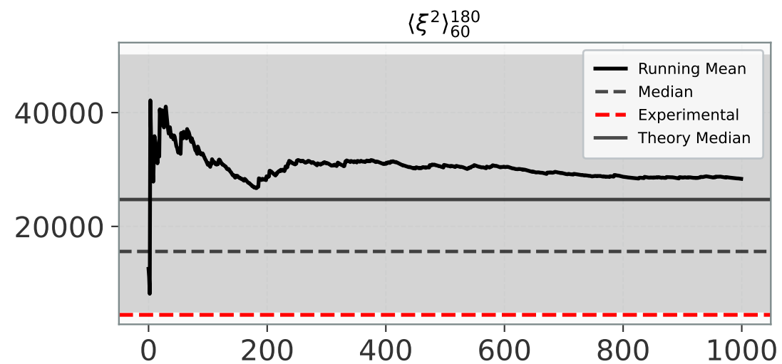
Convergence - base_omegak_CamSpecHM_TT_lowl_lowE
