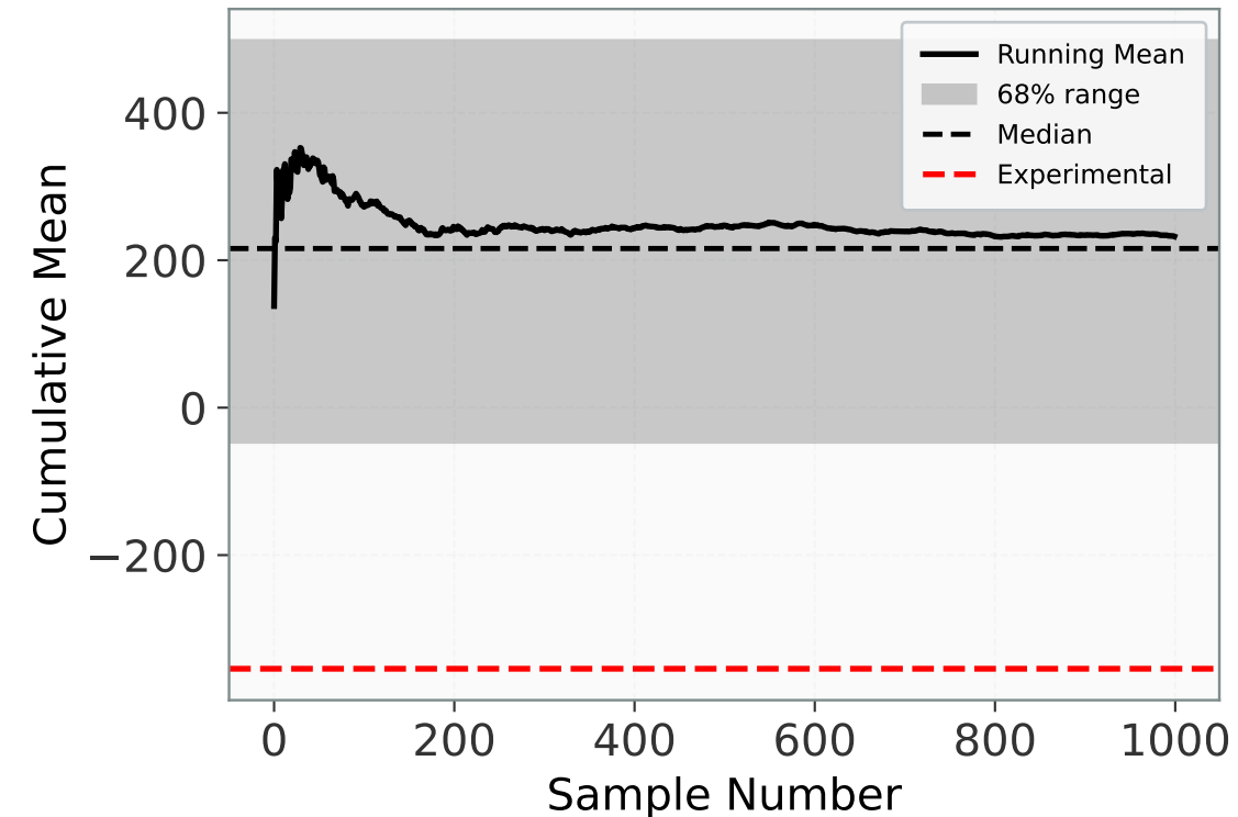
Convergence: \xi_{180}
