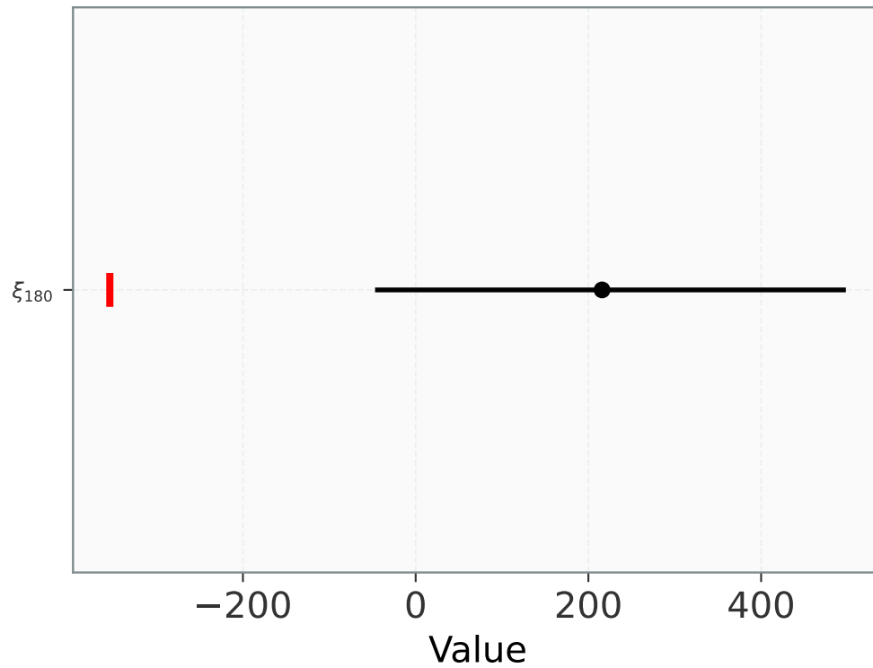
68% Credible Intervals
