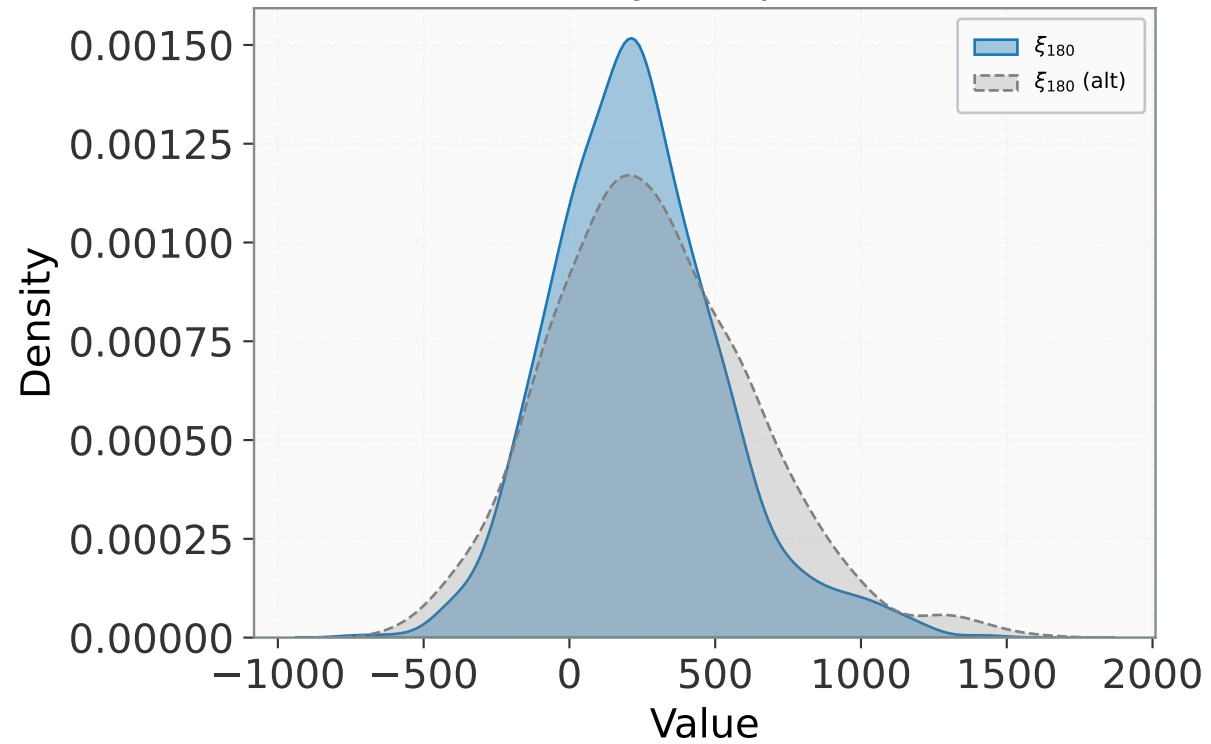
Density Comparison
