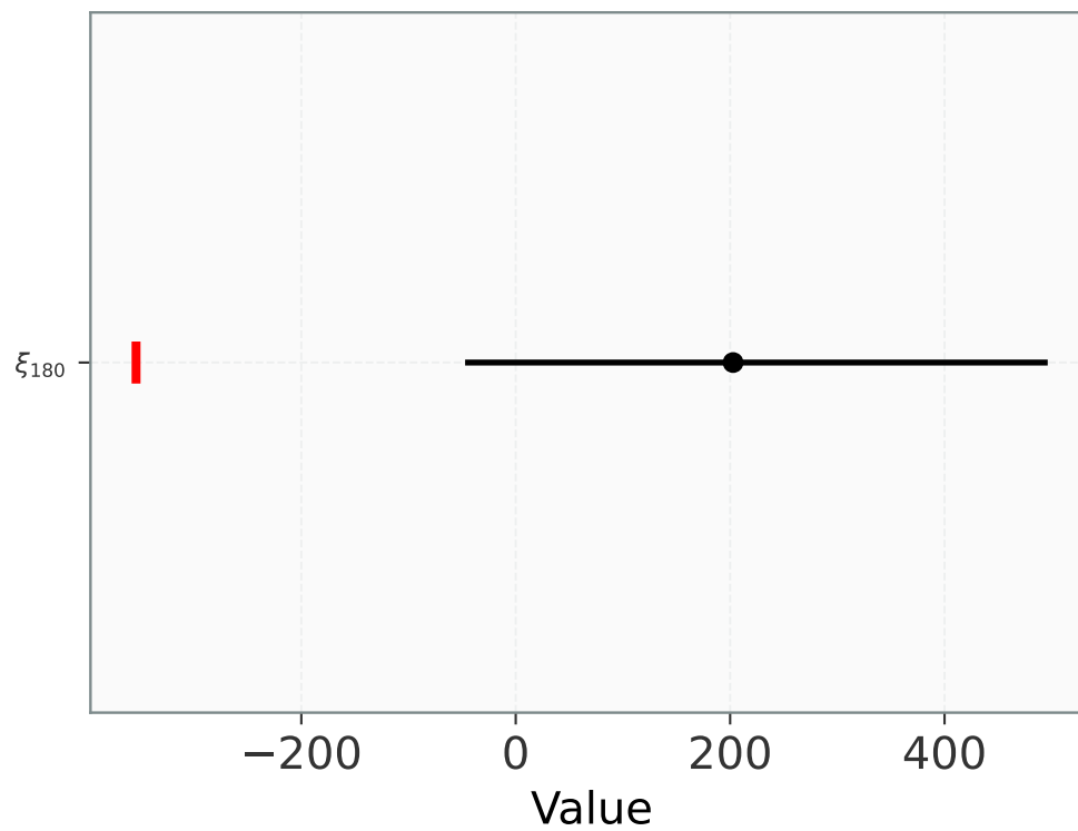
68% Credible Intervals
