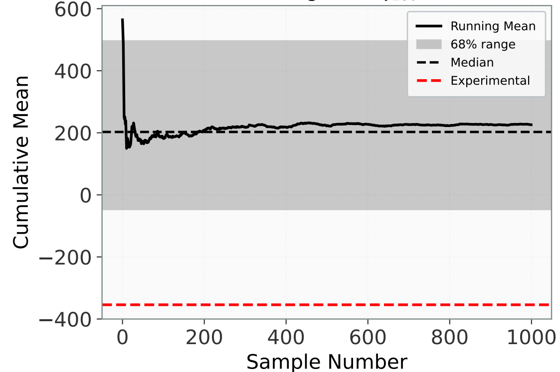
Convergence: \xi_{180}
