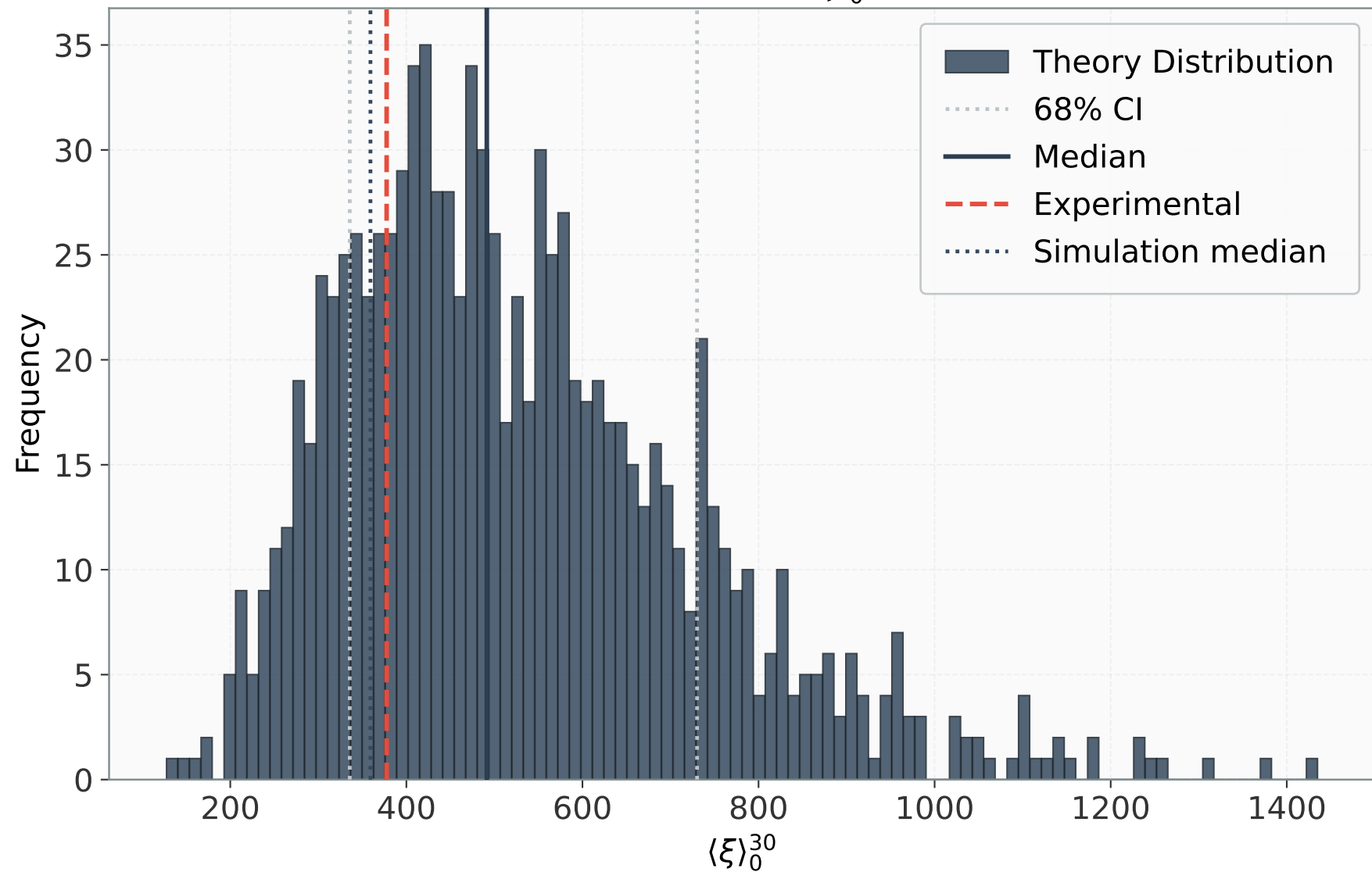
Distribution: \langle \xi \rangle_0^{30}
