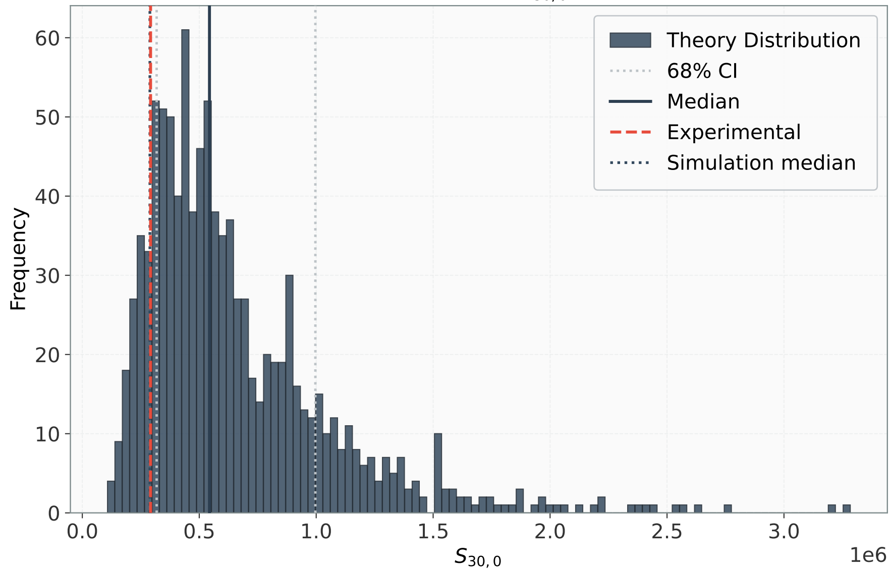
Distribution: S_{30,0}
