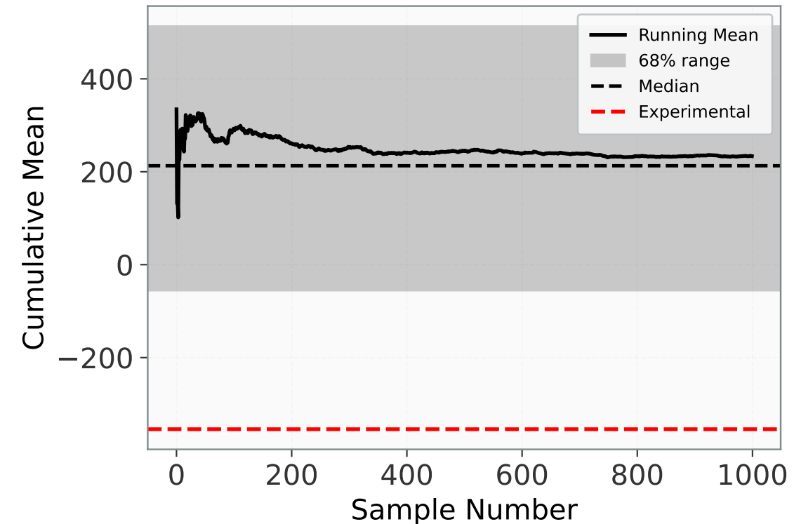
Convergence: C_{180}
