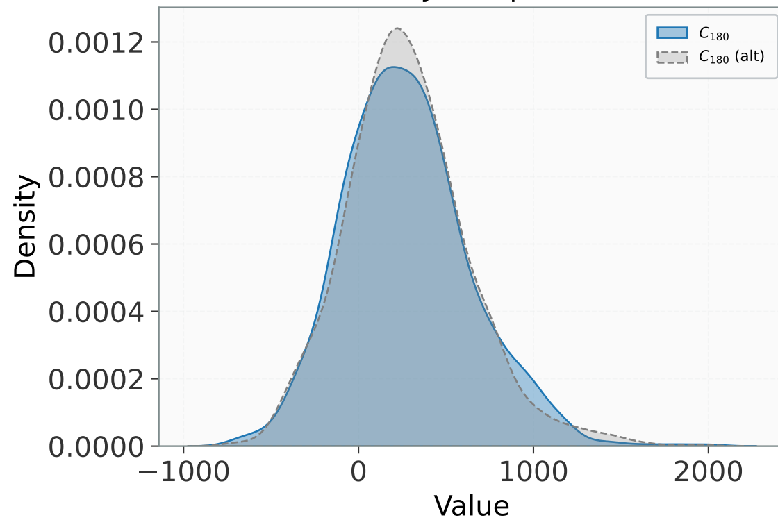
Density Comparison
