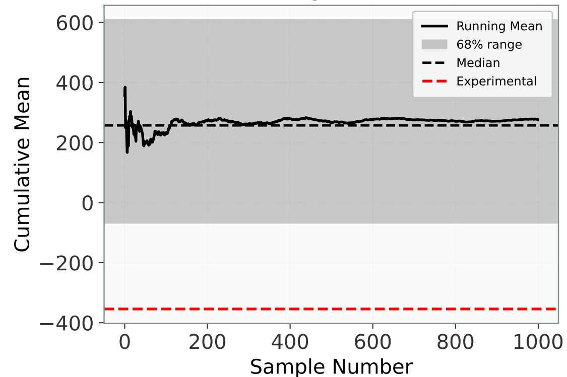
Convergence: C_{180}
