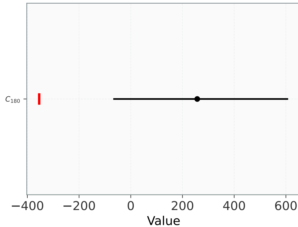
68% Credible Intervals
