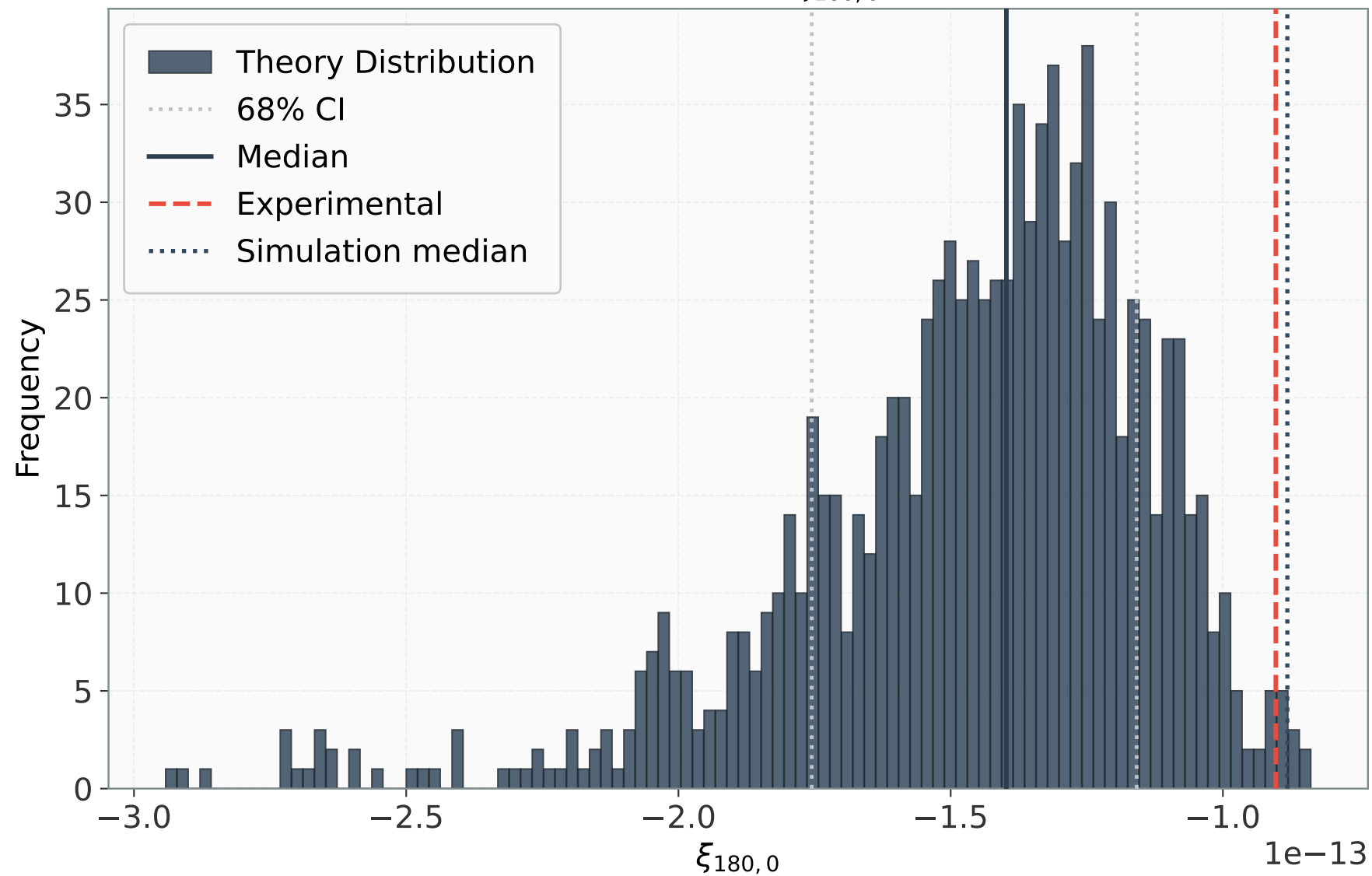
Distribution: \xi_{180,0}
