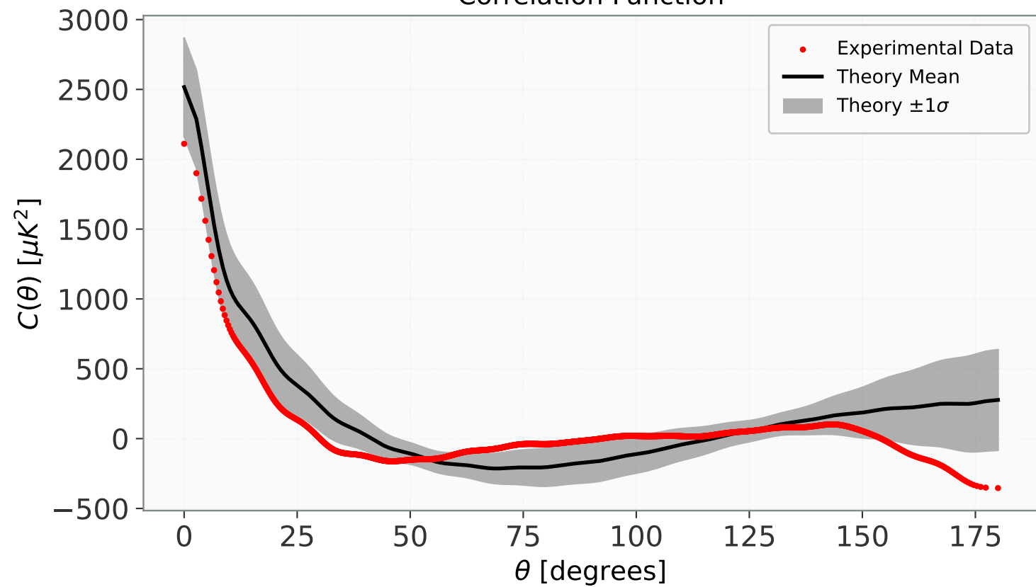
Correlation Function
