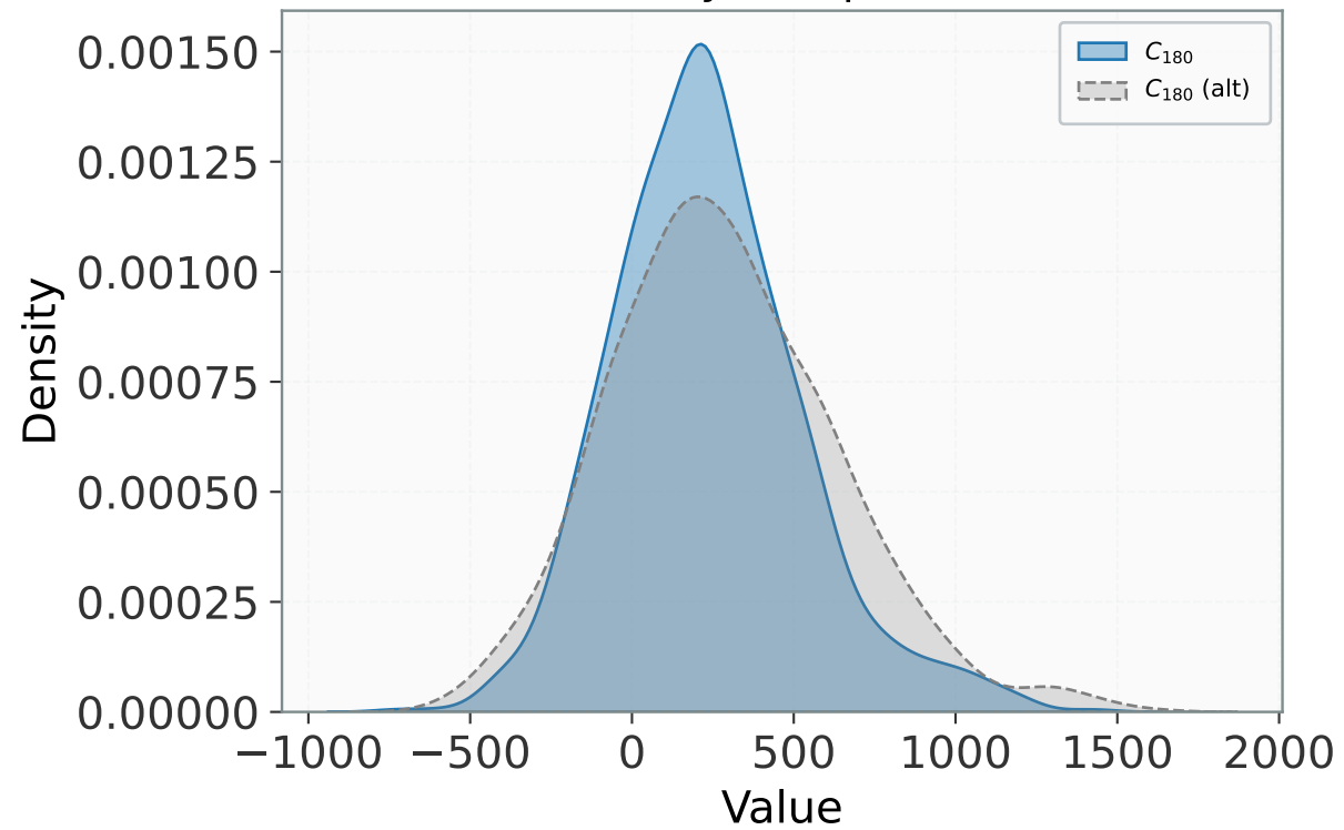
Density Comparison
