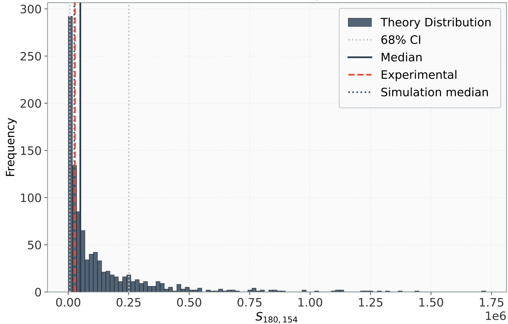
Distribution: S_{180,154}
